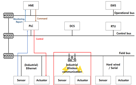
Fig. 1. Service scenario of industrial control system[15]
